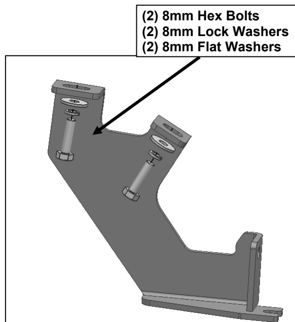
(Fig 2) Attach the Front Mounting Bracket to the front location
