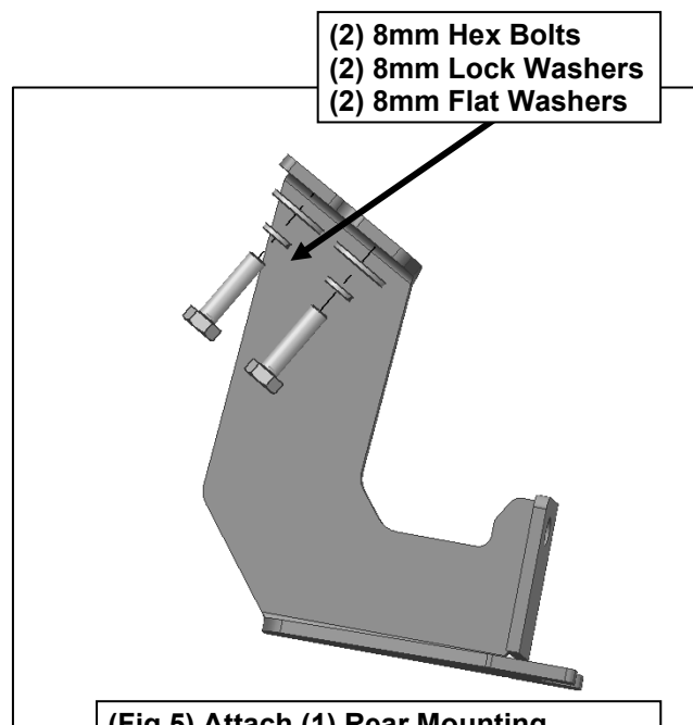
(Fig 5) Attach (1) Rear Mounting Bracket to the 2nd location
