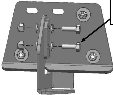
(Fig 3) Driver/Left Front mounting location
