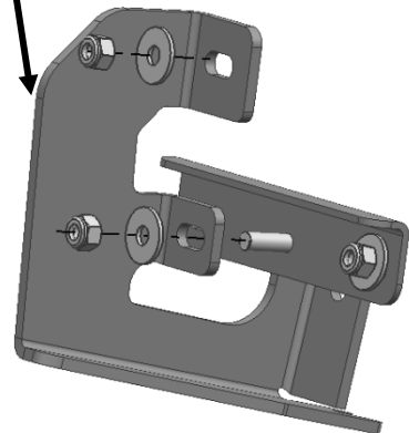
(Fig 6) Attach Mounting Bracket to the upper mounting stud and Support Bracket
