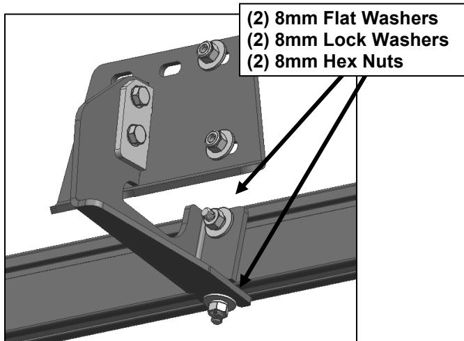
(Fig 13) Attach the Universal Mounting Tube to the Front/Rear Mounting Brackets.
